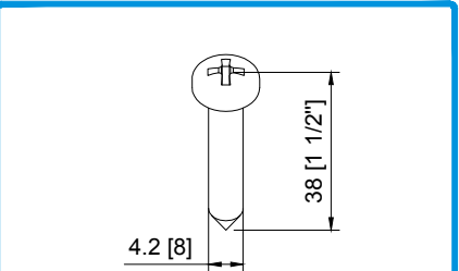
290030 PARAF. DIN7981 4,2x38 INOX A2
