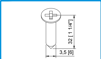
290080 PARAF. DIN7982 PH 3,5x32 INOX A2
