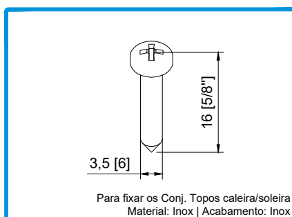
290729 PARAF PKI PH 5/8x6 CQ 290476
