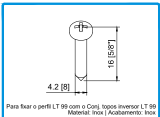
290088 PARAF. DIN7981 PH 4,2x16 INOX A2
