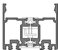
OS 69 Perfil móvel central Central mobile profile | Cadre ouvrant central
