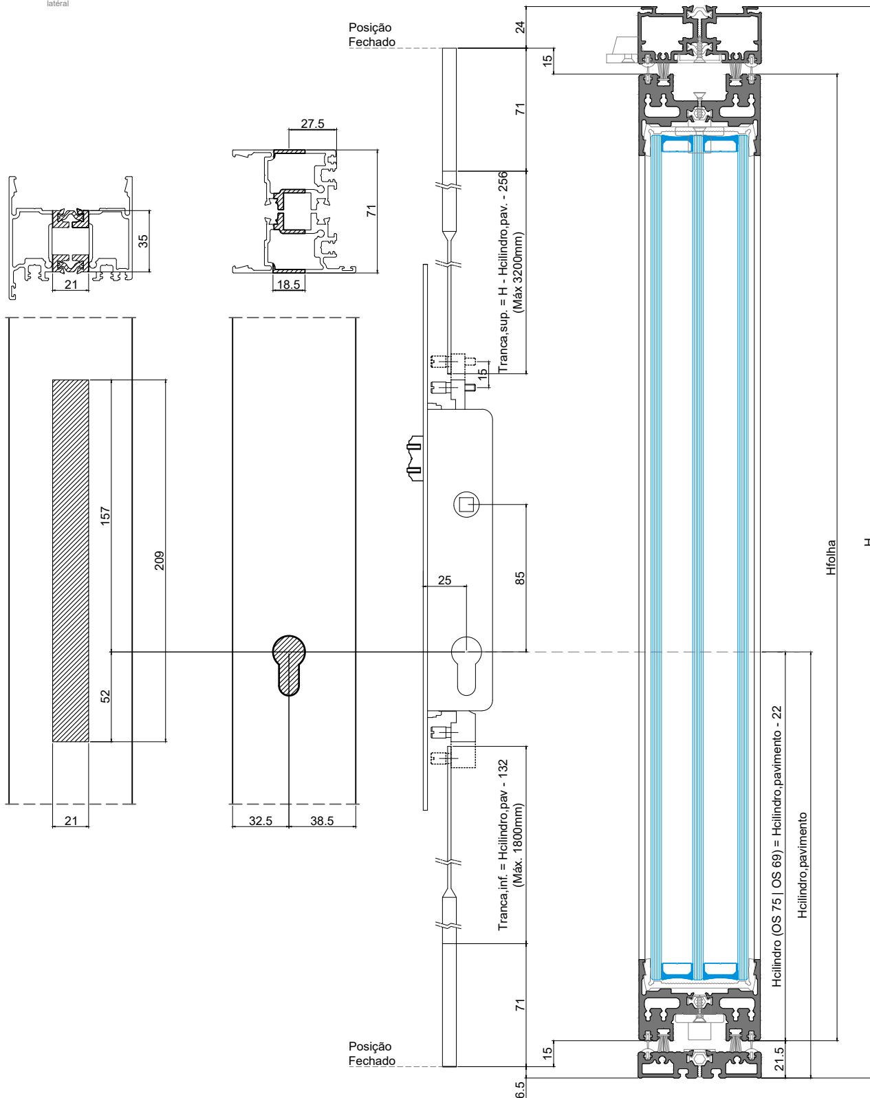
OS 69 Perfil móvel central Central mobile profile | Cadre ouvrant central
