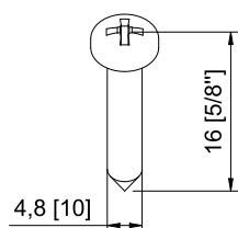
290064 PARAF. DIN7981 PH 4,8X16 INOX A2
